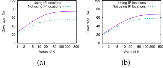
Fig. 13: Top- K coverage by TF-IDF similarities for Beijing (a) and Harbin (b).
