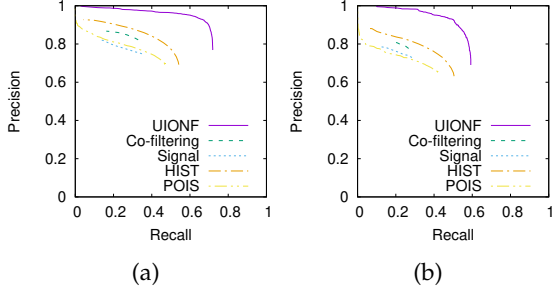
Fig. 12: Comparing our framework with baselines in (a) for Beijing and (b) for Harbin, using only the subset of the whole dataset which appears in the ground truth.
